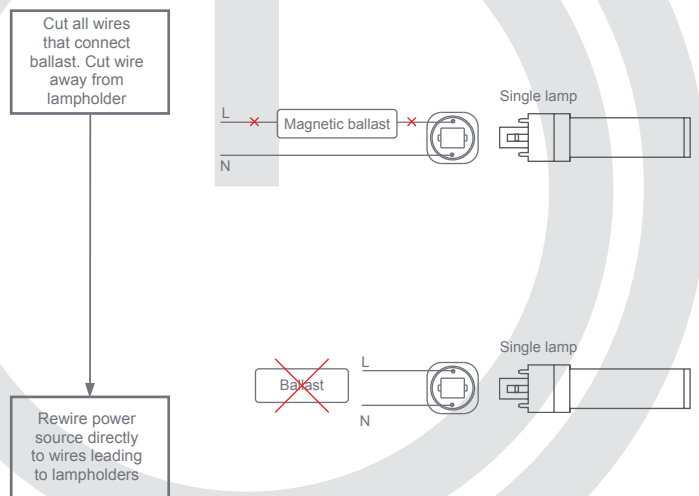
Diagram 2 – Magnetic ballast fixture wiring modification
